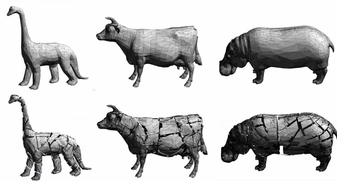
Fig. 6. BSP solid models from B-rep triangulations, and exploded views of the cell complexes.
