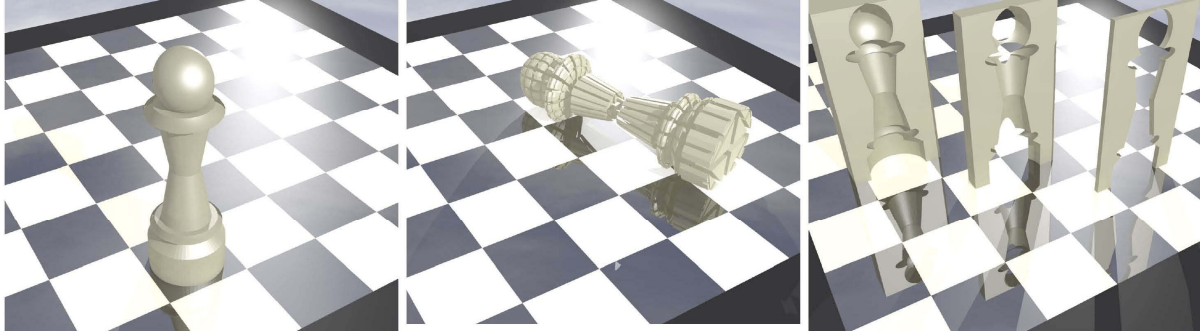
Fig. 2. A chess model: (a) union of a cylinder, a cone, a scaled sphere, two cones, a scaled sphere and a sphere, rendered flat at maximum resolution; (b) exploded geometry; (c) differences from parallelepipeds.
