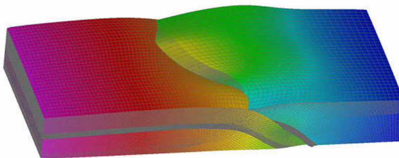
Fig. 7. Computational simulation result of Tokai region in Japan by CHIKAKU STATIC. A hexahedral mesh is generated by CHIKAKU MESH.
