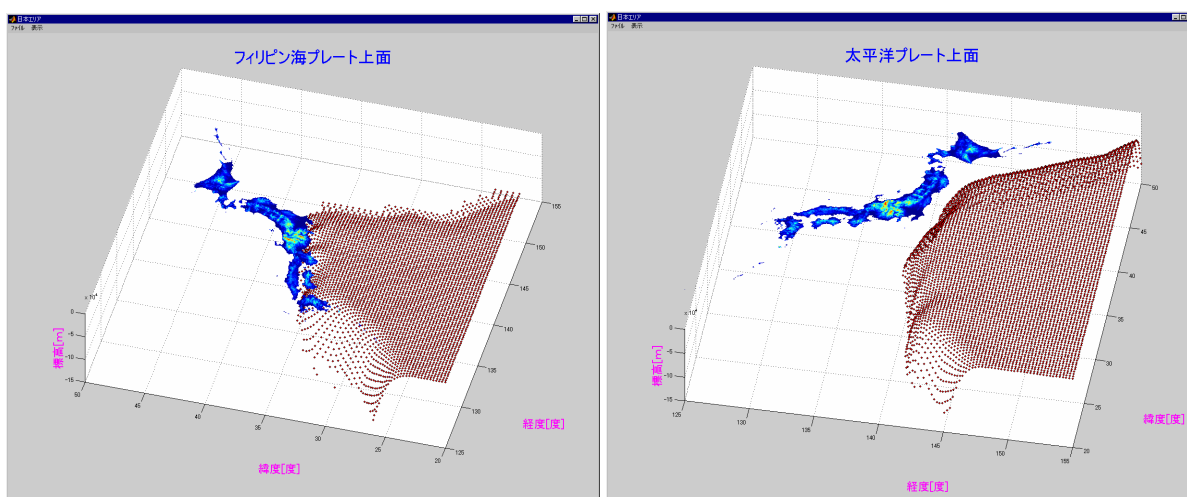
Fig. 5. Display results of grid polygons for plate surfaces. Left: Philippine Sea plate. Right: Pacific plate.
