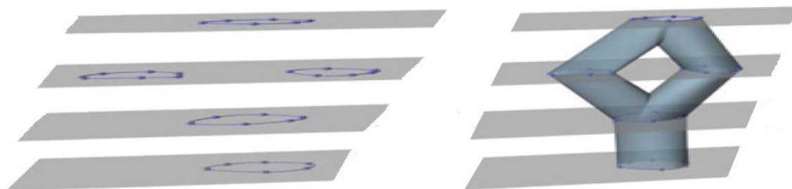
Figure 1: Interpolating surface construction: (a) the contour data set on parallel planes (b) one possible interpolating surface.
