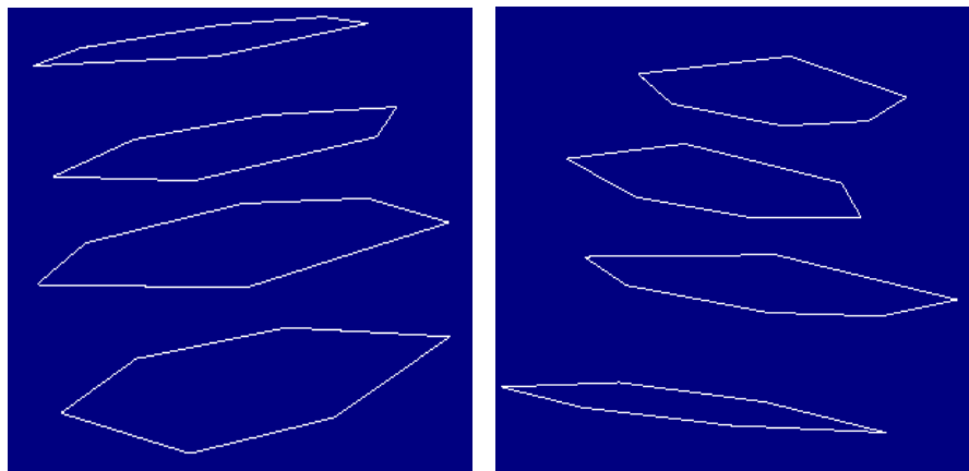
Figure 7: Initial contours: (a) example1 (b) example2.
