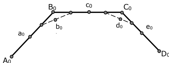
Figure 2: Uniform cubic refinement of a polygon.
