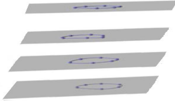
Figure 6: Interpolating surface construction in a simplified case.
