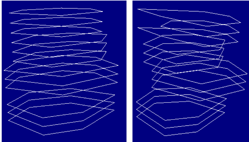
Figure 8: Augmented contours: (a) example1 (b) example2.
