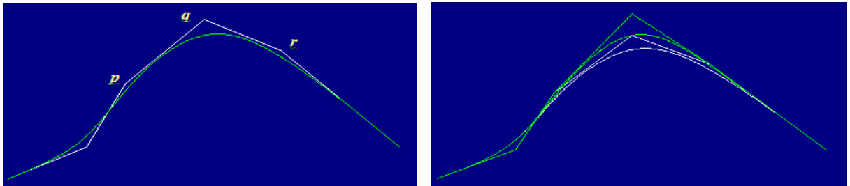
Figure 3: Interpolating points by curves: (a) initial control polygon and curve (b) polygon modified to interpolate a given point.
