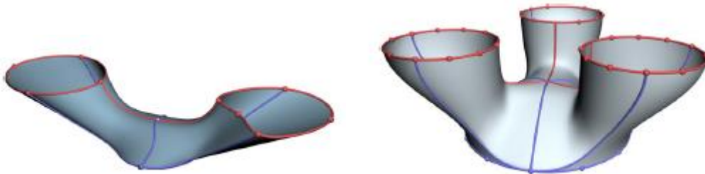
Figure 11: Branching as tackled by Gabrielides et al. [3]: (a) The final “one-to-two” surface (b) The final “one-to-three” branching surface.
