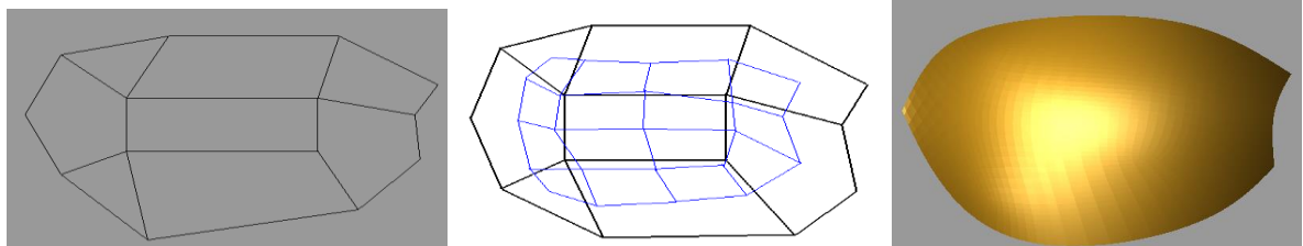
Figure 4: Catmull-Clark subdivision: (a) initial control mesh (b) a single subdivision step and (c) the limit surface.
