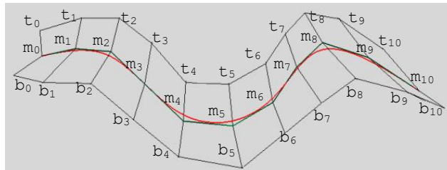
Figure 5: A Catmull-Clark polygonal complex.
