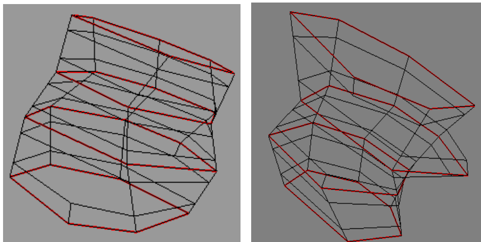
Figure 9: Control mesh generation: (a) example1 (b) example2.
