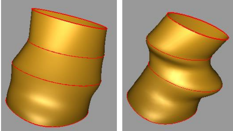
Figure 10: Interpolating surface.
