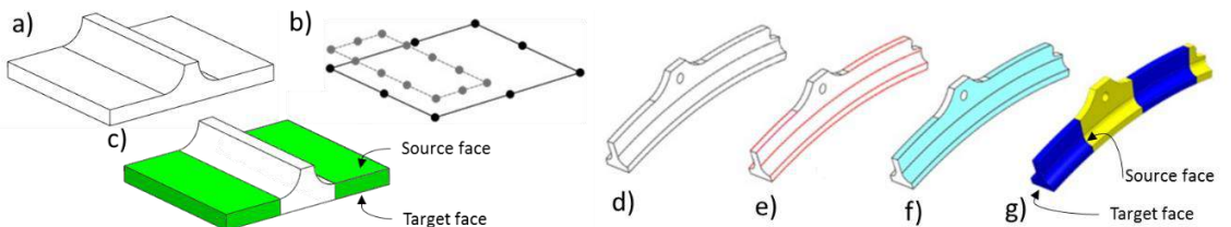
Figure 2: Thin-sheet [17] (left) and long-slender [18] (right) decomposition: (a) candidate geometry, (b) discretized face pair, (c) two thin-sheet regions extracted in green, (d) candidate geometry, (e) long-edges identification, (f) 2 loops of long faces, and (g) two long-slender regions extracted in blue.
