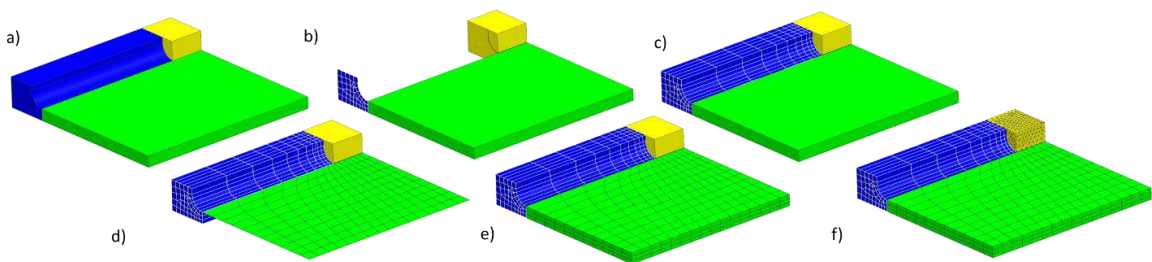
Figure 9: Meshing sequence for a simple component.
