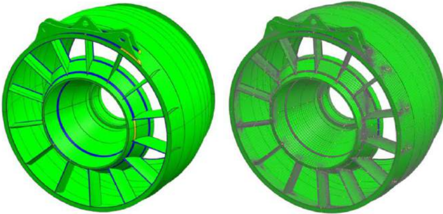
Figure 12: Decomposition and mesh of a turbine casing.
